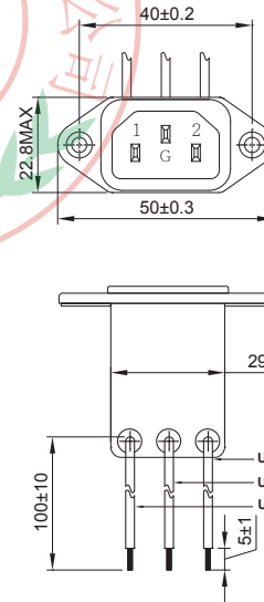
YA-T (Lead-wire)
