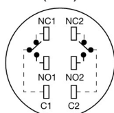
按钮开关/Push Button (TOP)
