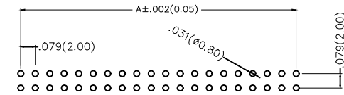
Recommended P.C.Board Layout
