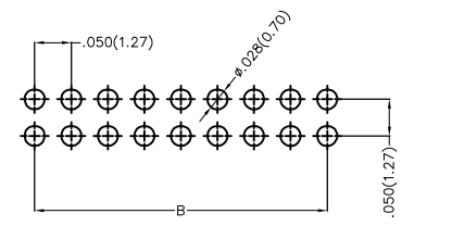
Recommended P.C.Board Layout Tolerances: ±.002(0.05)
