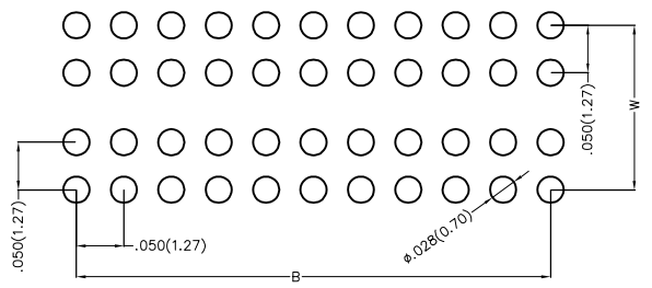
Recommended P.C.Board Layout Tolerances: ±.002(0.05)
