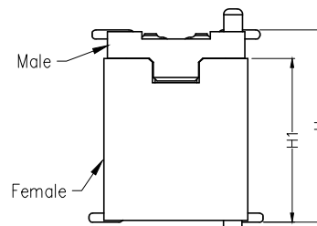
ASSEMBLY
