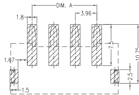
Mating PCB detail I
