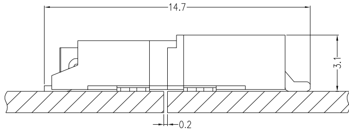
Assembly Layout
