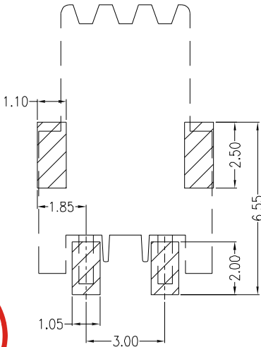
Board Layout
