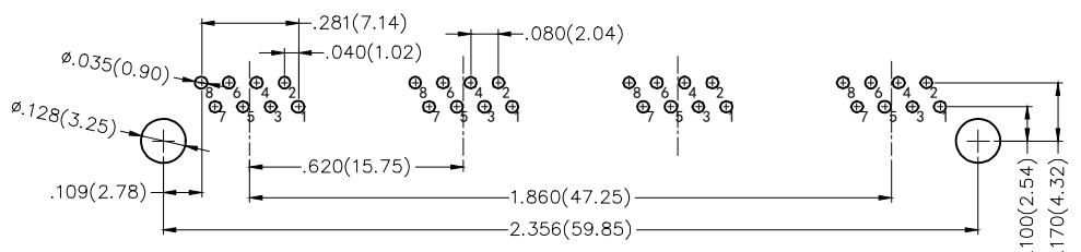
Recommended P.C.Board Layout Tolerances: ±.002(0.05)
