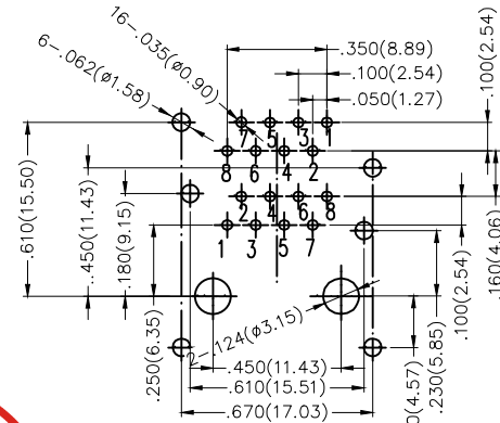
Recommended P.C. Board layout (Tolerances±.002(0.05))
