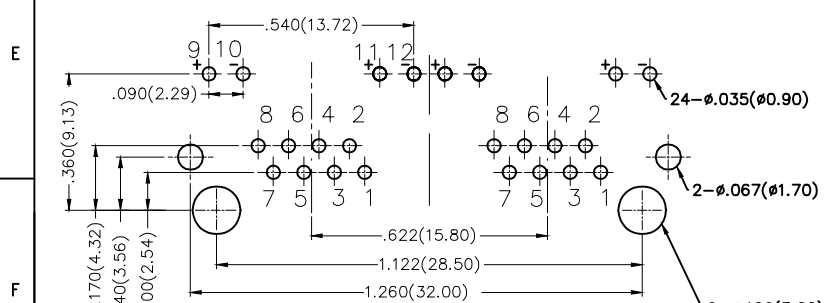
Recommended P.C.Board Layout Tolerances: ±.002(0.05)
