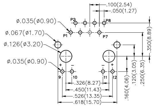
Recommended P.C.Board Layout Tolerances: ±.002(0.05)
