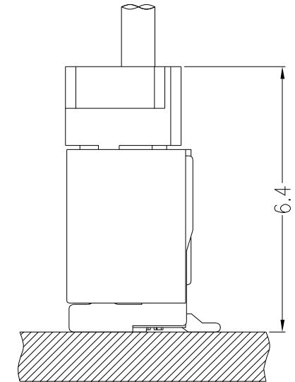
Assembly Layout
