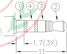
∅2.5 SPECIAL MATE PLUG
