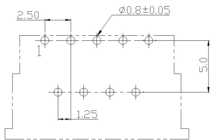
RECOMMEND PCB LAYOUT COMPONENT SIDE (FOR:GS15-XX1XAW)
