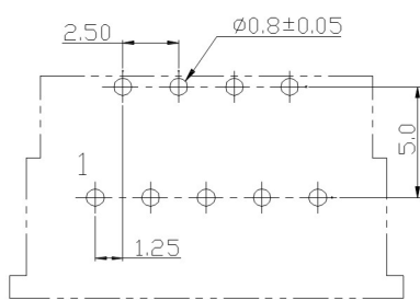
RECOMMEND PCB LAYOUT COMPONENT SIDE (FOR:GS15-XX1XA)
