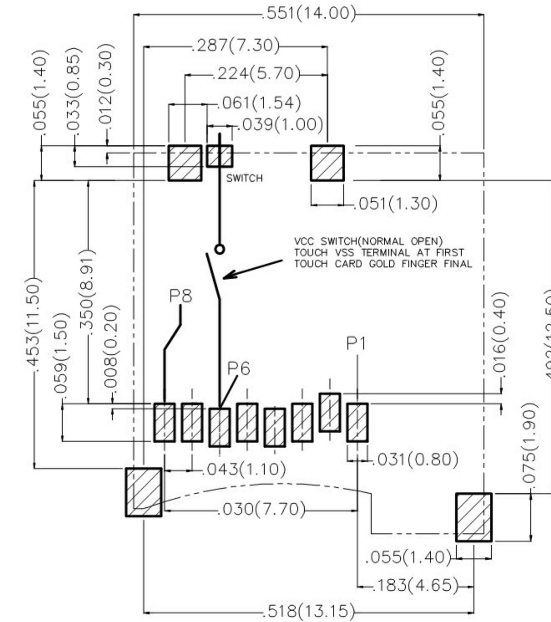
Recommended P.C.Board Layout
