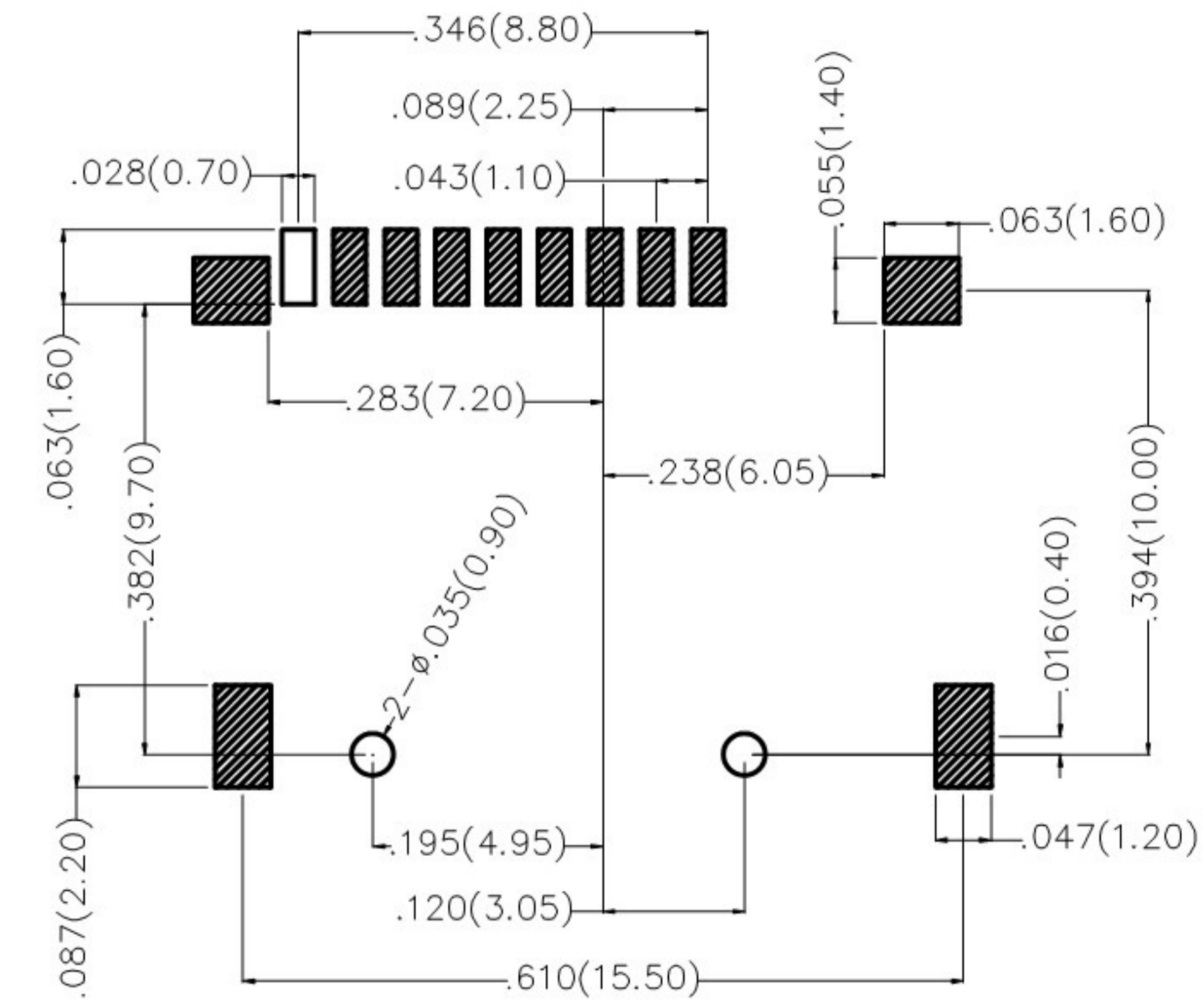
Recommended P.C.Board Layout
