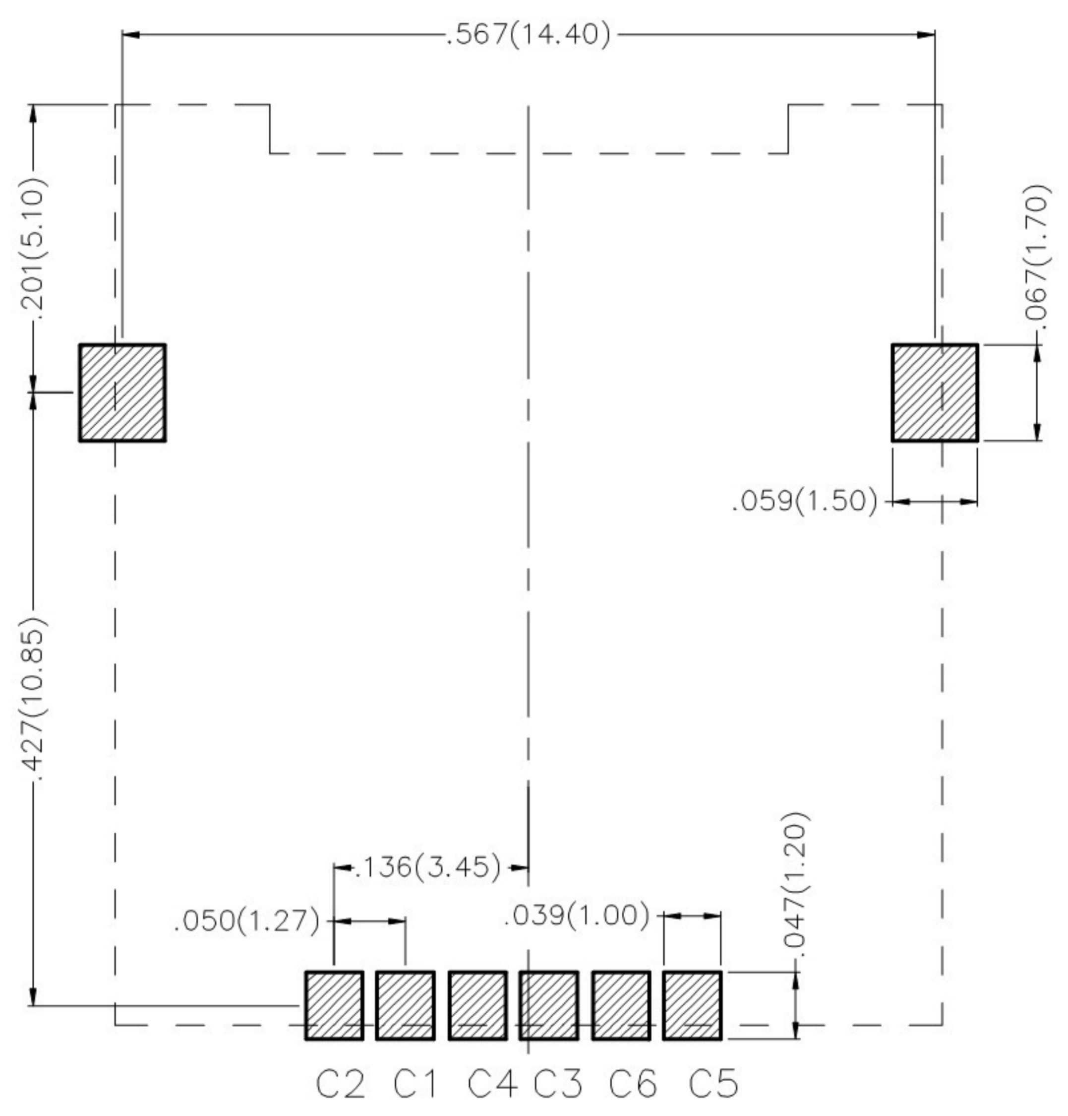
Recommended P.C.Board Layout General Tolerances: ±0.05
