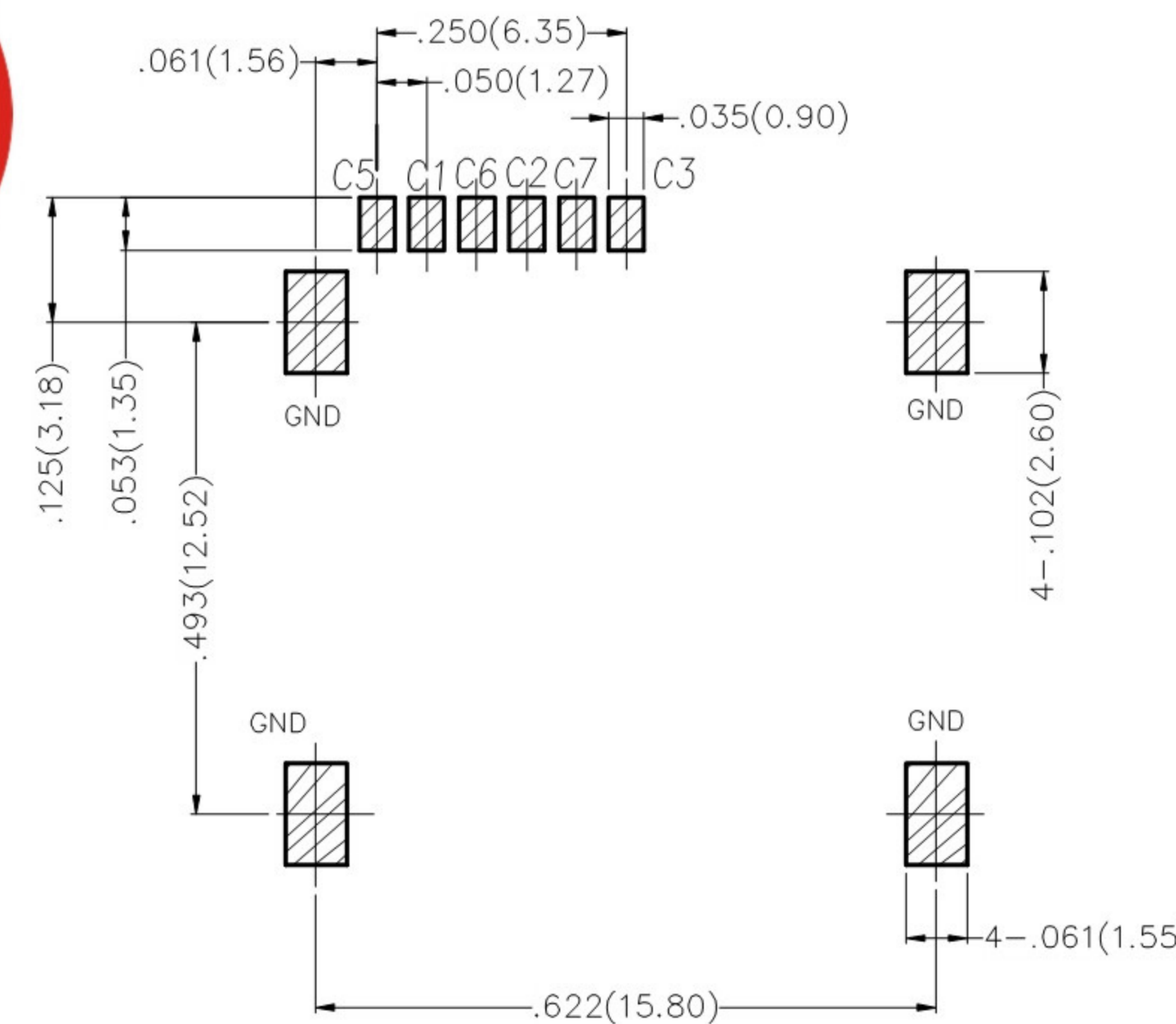
Recommended P.C.Board Layout GENERAL TOLERANCES: ±0.05mm
