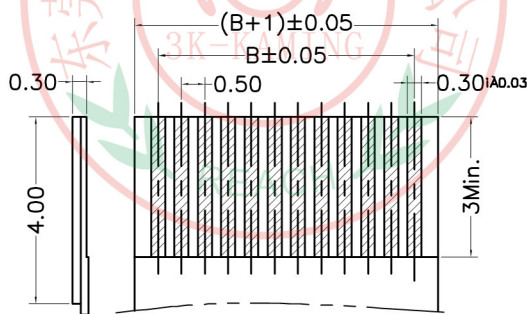
Applicable FPC
