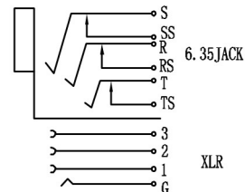
SCHEMATIC
