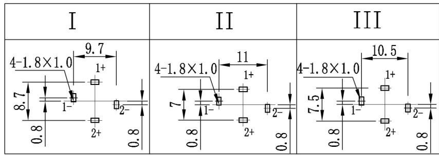
PCB LAYOUT Vertical view
