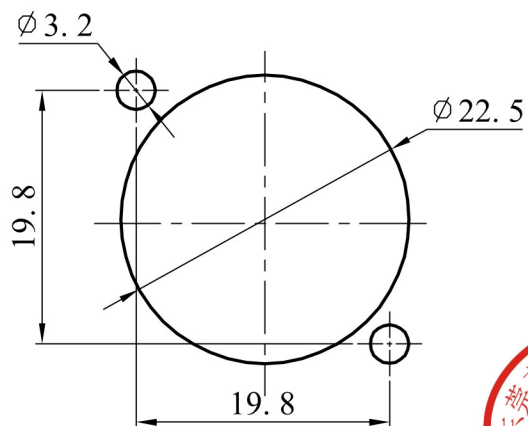
PANEL CUTOUT
