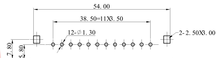
PCB LAYOUT
