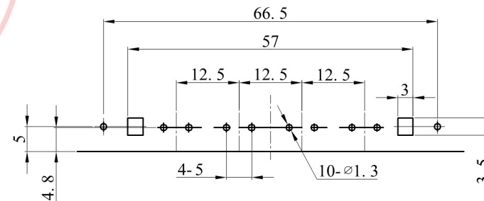
PCB LAYOUT
