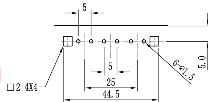
PCB-MTG (Solder Surface) TOP VIEW
