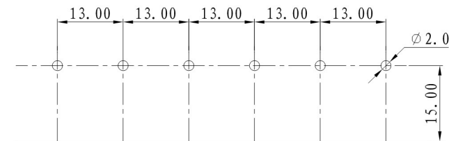
PCB LAYOUT TOP VIEW TOP VIEW
