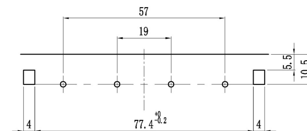
PCB-MTG TOP VIEW
