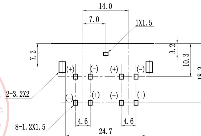
PCB MOUNTING HOLES (Solder surface) TOP VIEW
