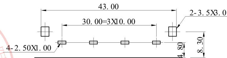
PCB LAYOUT
