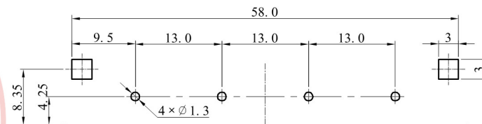
PCB LAYOUT
