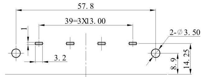
PCB LAYOUT
