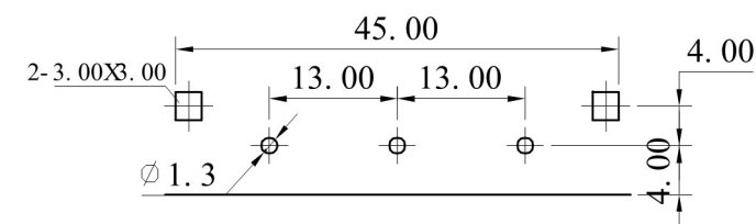
PCB LAYOUT
