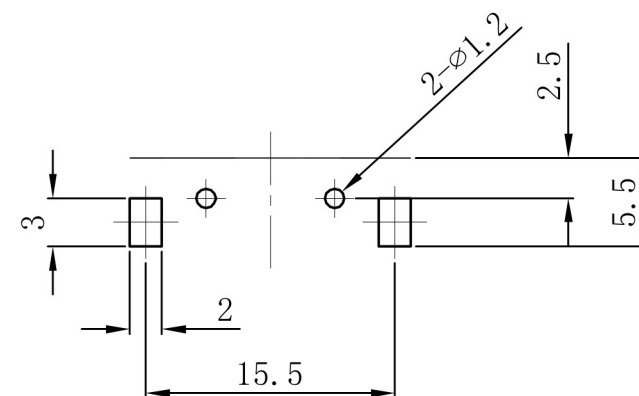
PCB-MTG (Solder Surface) TOP VIEW
