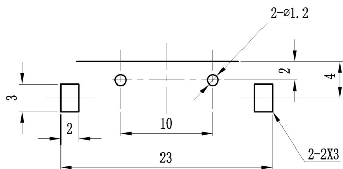
PCB-MTG (Solder Surface) TOP VIEW
