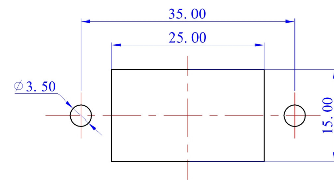
Installation Dimensions
