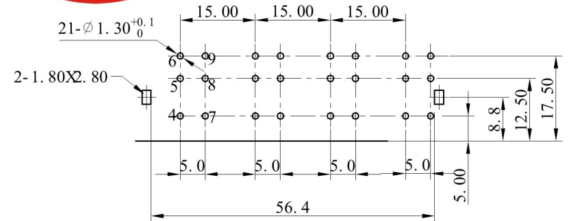
PCB TOP VIEW
