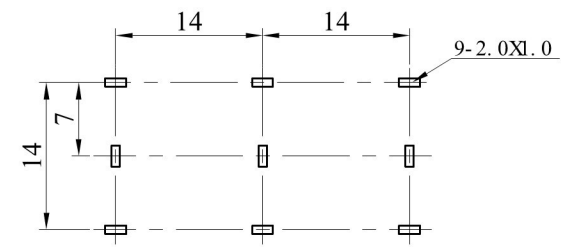
PCB LAYOUT TOP VIEW
