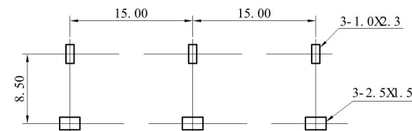
PCB LAYOUT TOP VIEW
