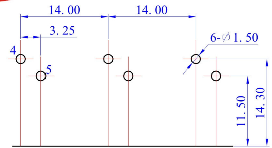
PCB TOP VIEW
