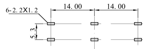
PCB LAYOUT TOP VIEW
