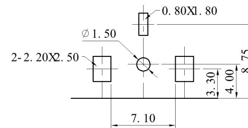
PCB TOP VIEW
