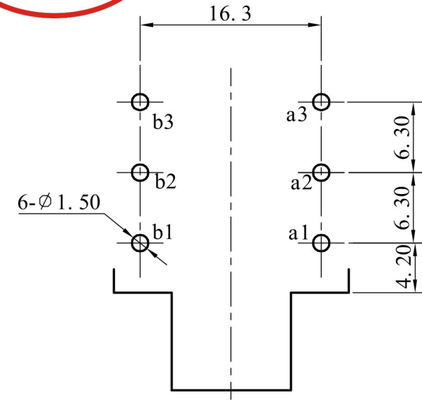
PCB LAYOUT
