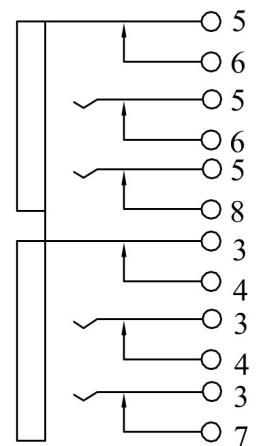
SCHEMATIC
