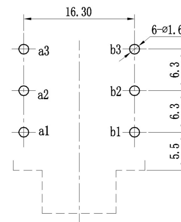
PCB LAYOUT
