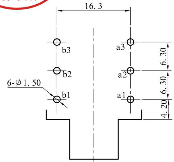
PCB LAYOUT
