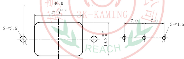
PANEL CUT-OUT
