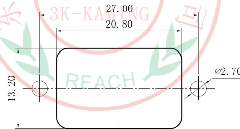
PANEL CUT-OUT
