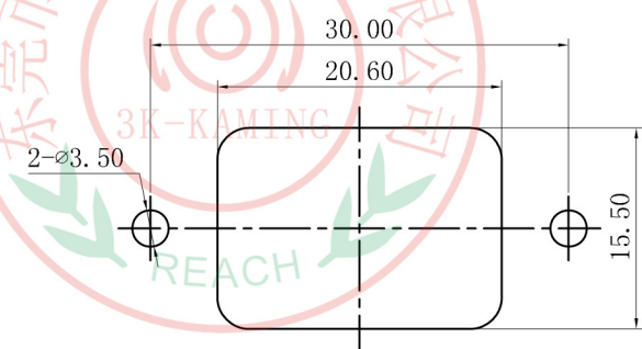
PANEL CUT-OUT
