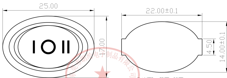
PANEL CUT-OUT
